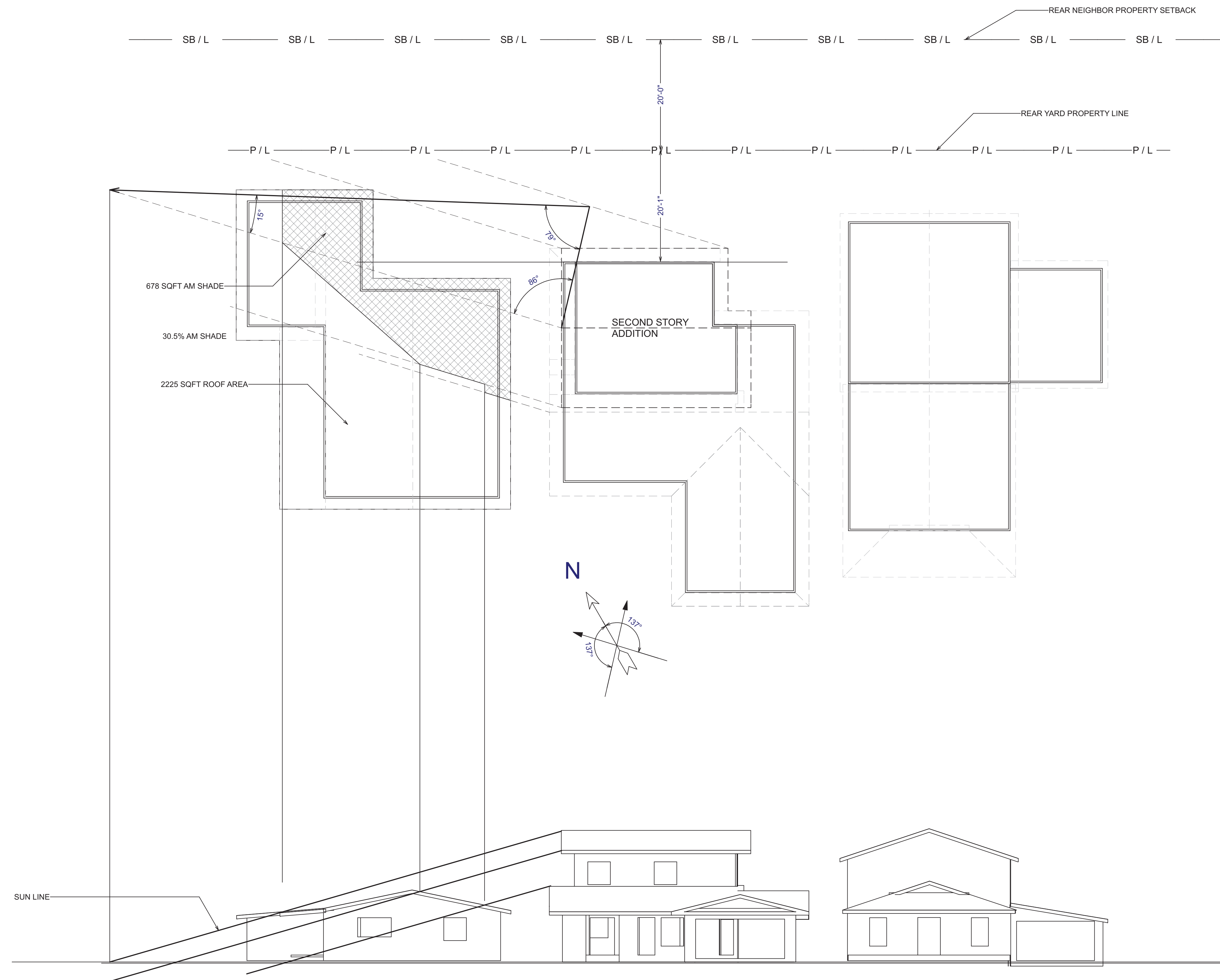
1 SOLAR STUDY AM A-05 SCALE = 1/10 in = 1 ft
